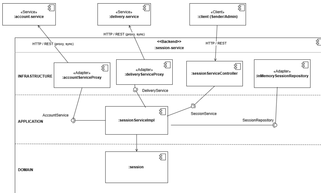
C&C diagram del session service
